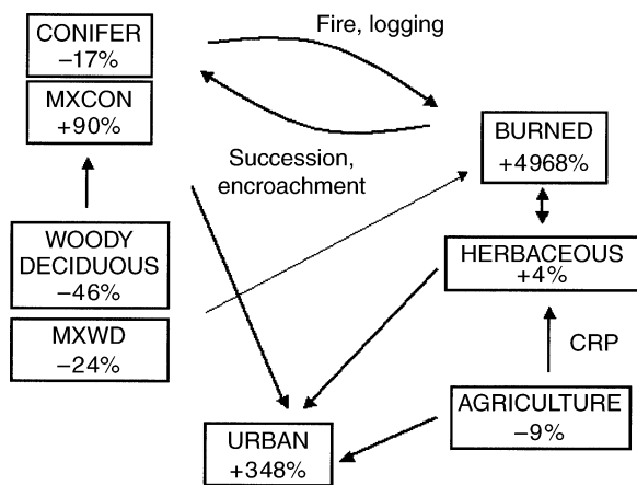
FIG. 4. Pathways of net gains and losses of percent cover change in the Greater Yellowstone Ecosystem, 1975–1995. MXWD = mixed woody deciduous/herbaceous, MXCON = mixed conifer/herbaceous.
